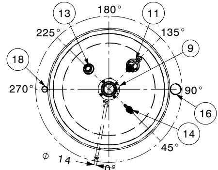
Detail C
