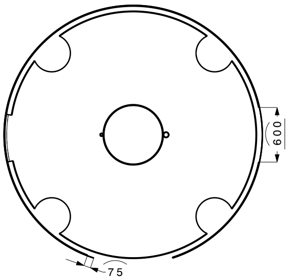
Section view L-L Scale: 1:42
