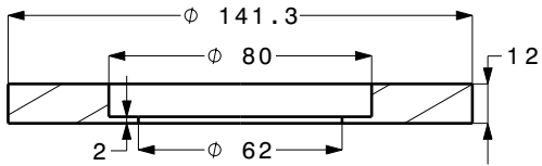
Section view X-X Scale: 2:5
