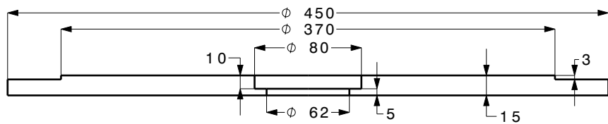
Section view T-T Scale: 1:4
