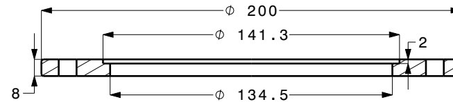
Section view W-W Scale: 2:5
