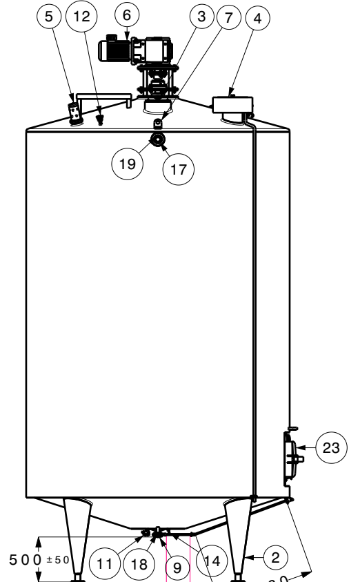
Left View
