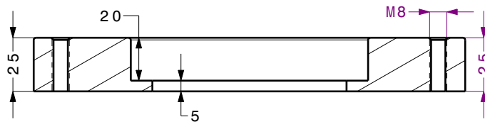
Section view V-V Scale: 2:5
